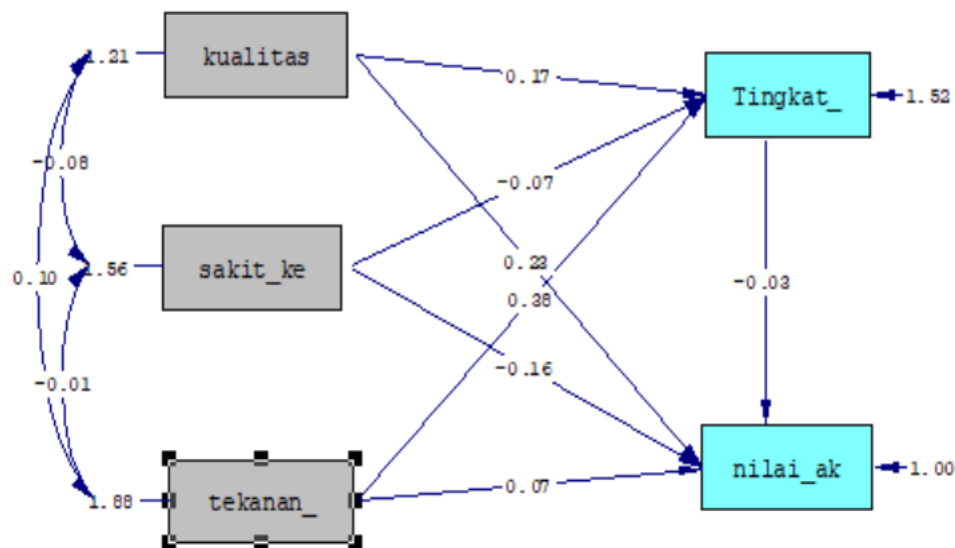
Gambar 1. Path Diagram 1
